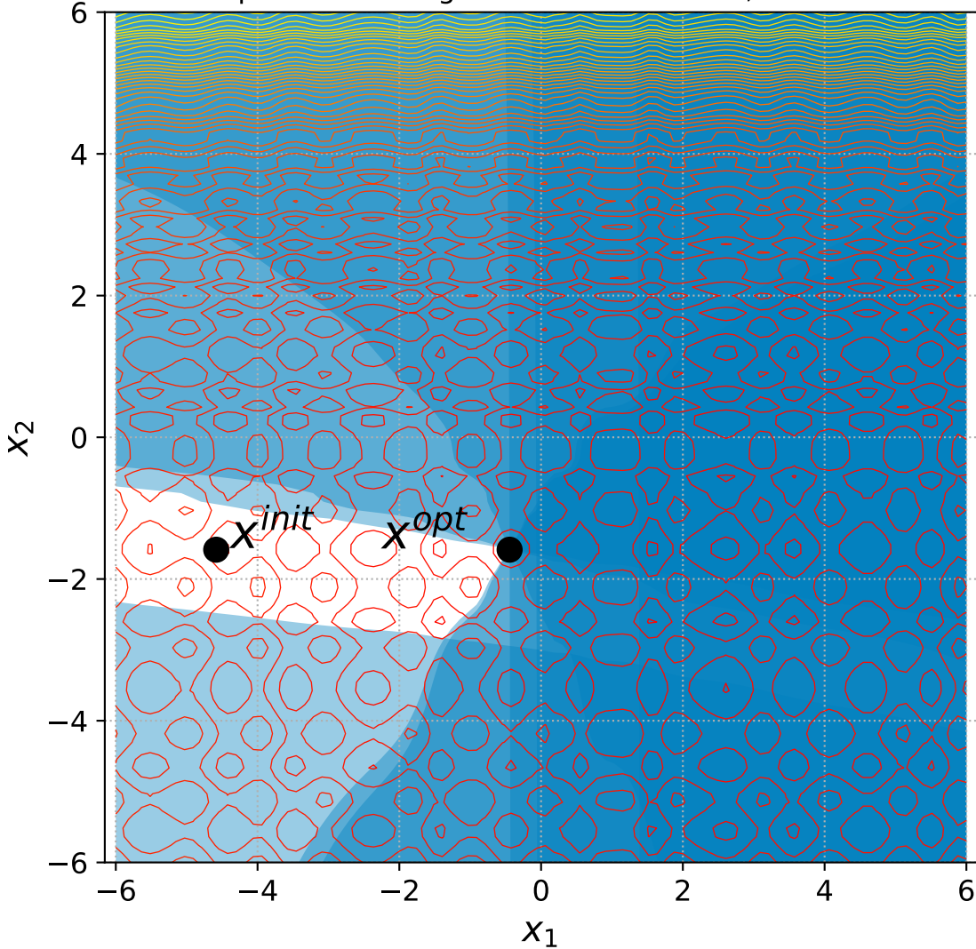
45 Separable Rastrigin with 6 constraints, instance=9
