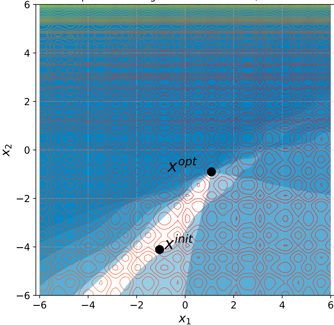
45 Separable Rastrigin with 6 constraints, instance=8
