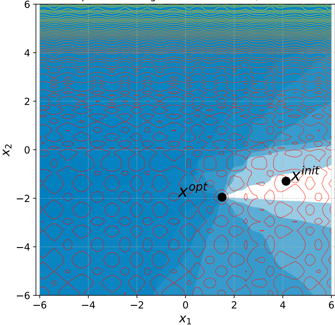
45 Separable Rastrigin with 6 constraints, instance=5
