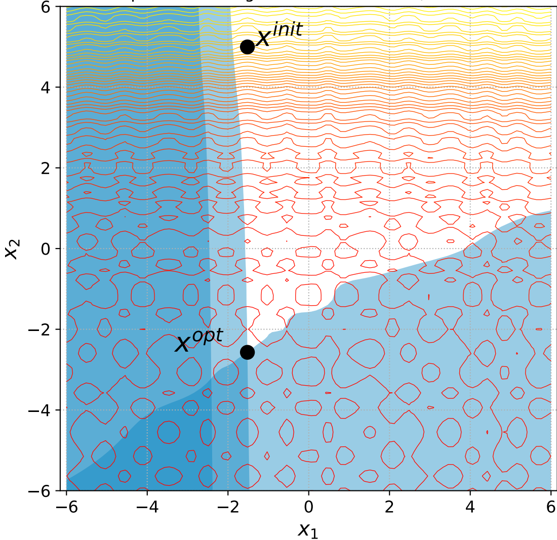
44 Separable Rastrigin with 2 constraints, instance=15
