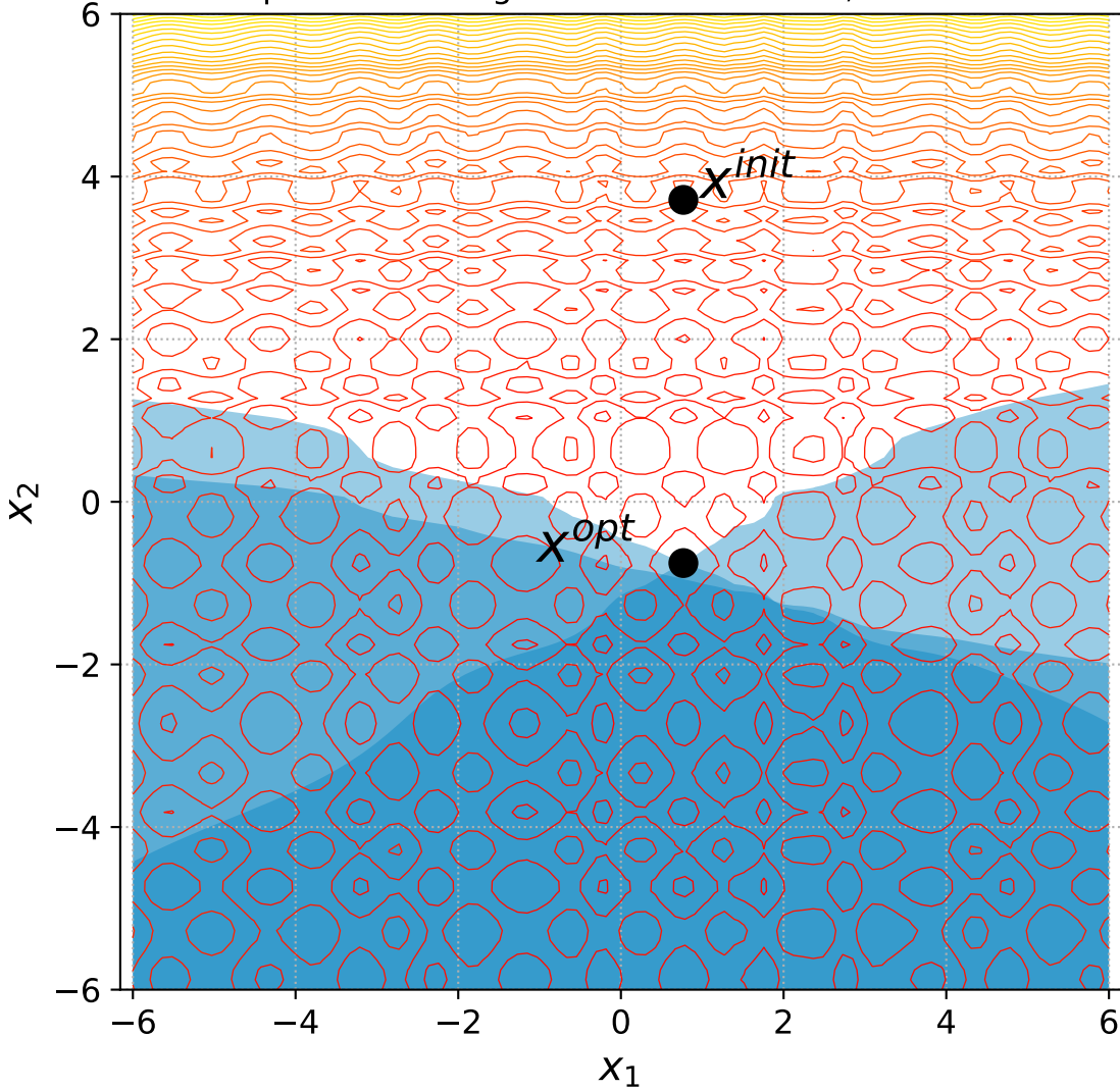
44 Separable Rastrigin with 2 constraints, instance=14
