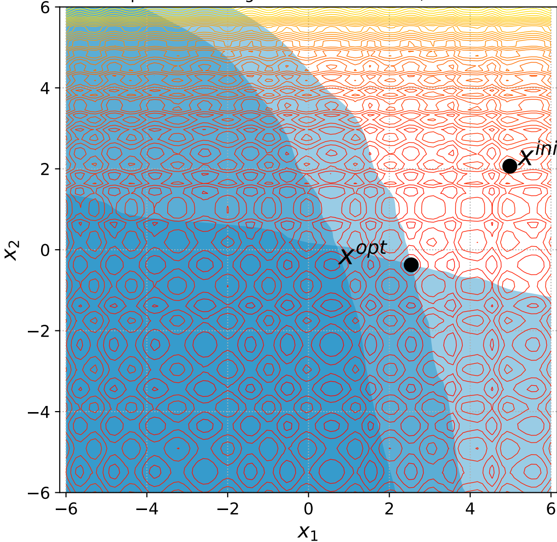
44 Separable Rastrigin with 2 constraints, instance=11
