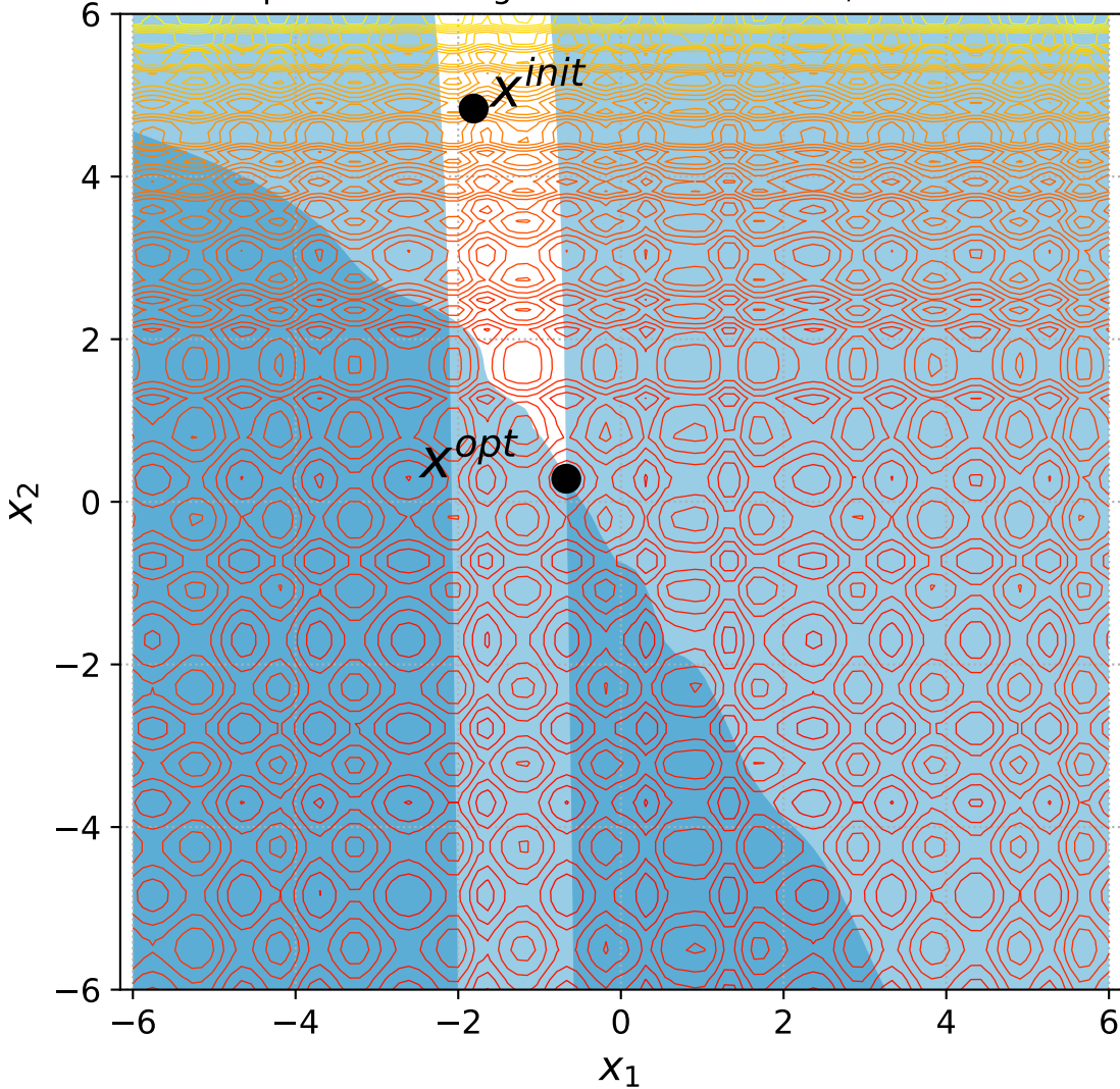
44 Separable Rastrigin with 2 constraints, instance=10
