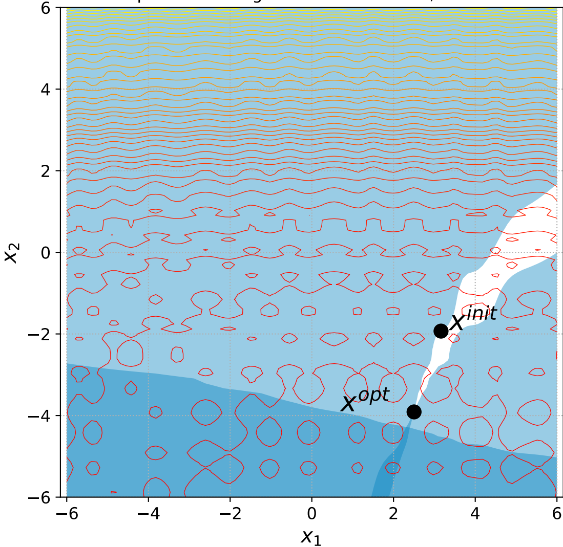
44 Separable Rastrigin with 2 constraints, instance=9
