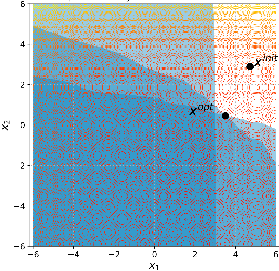
44 Separable Rastrigin with 2 constraints, instance=8
