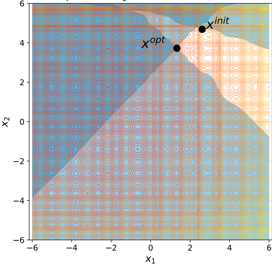
44 Separable Rastrigin with 2 constraints, instance=7
