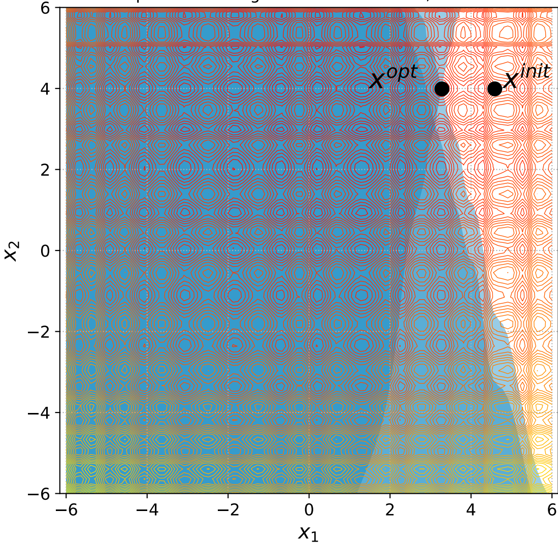
44 Separable Rastrigin with 2 constraints, instance=6
