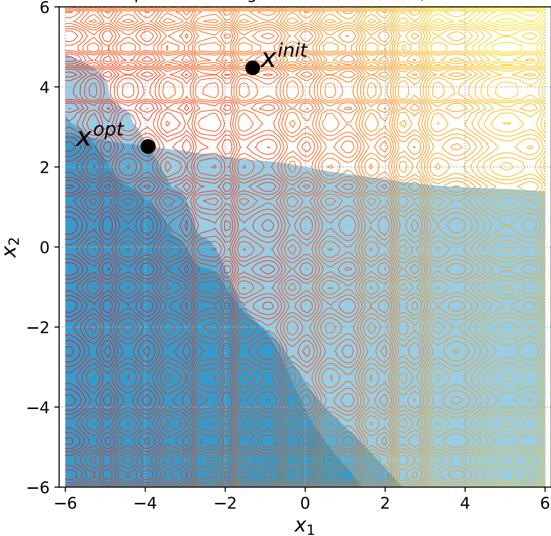
44 Separable Rastrigin with 2 constraints, instance=5
