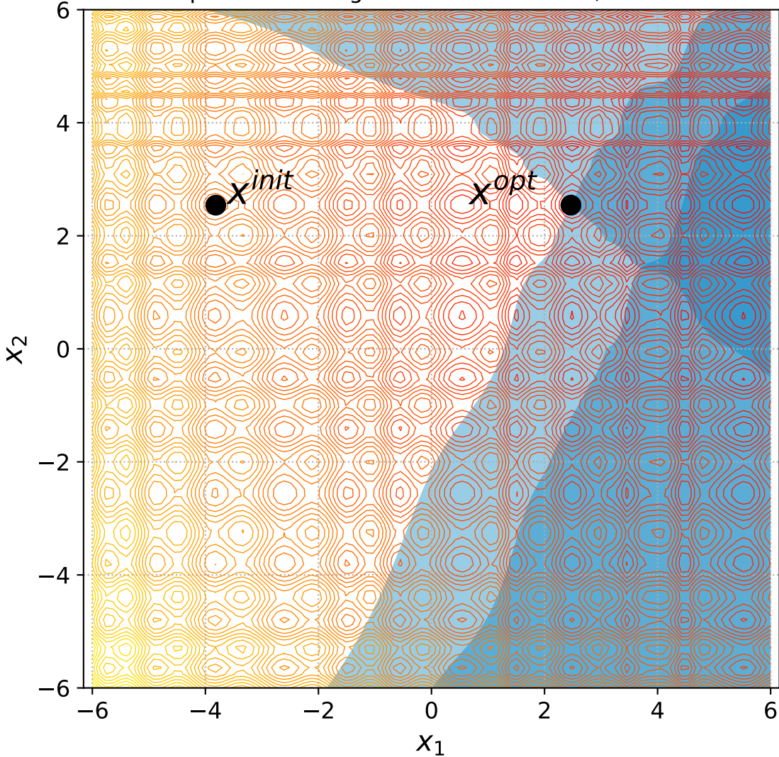
44 Separable Rastrigin with 2 constraints, instance=4
