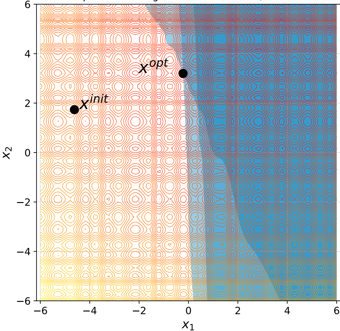
44 Separable Rastrigin with 2 constraints, instance=1
