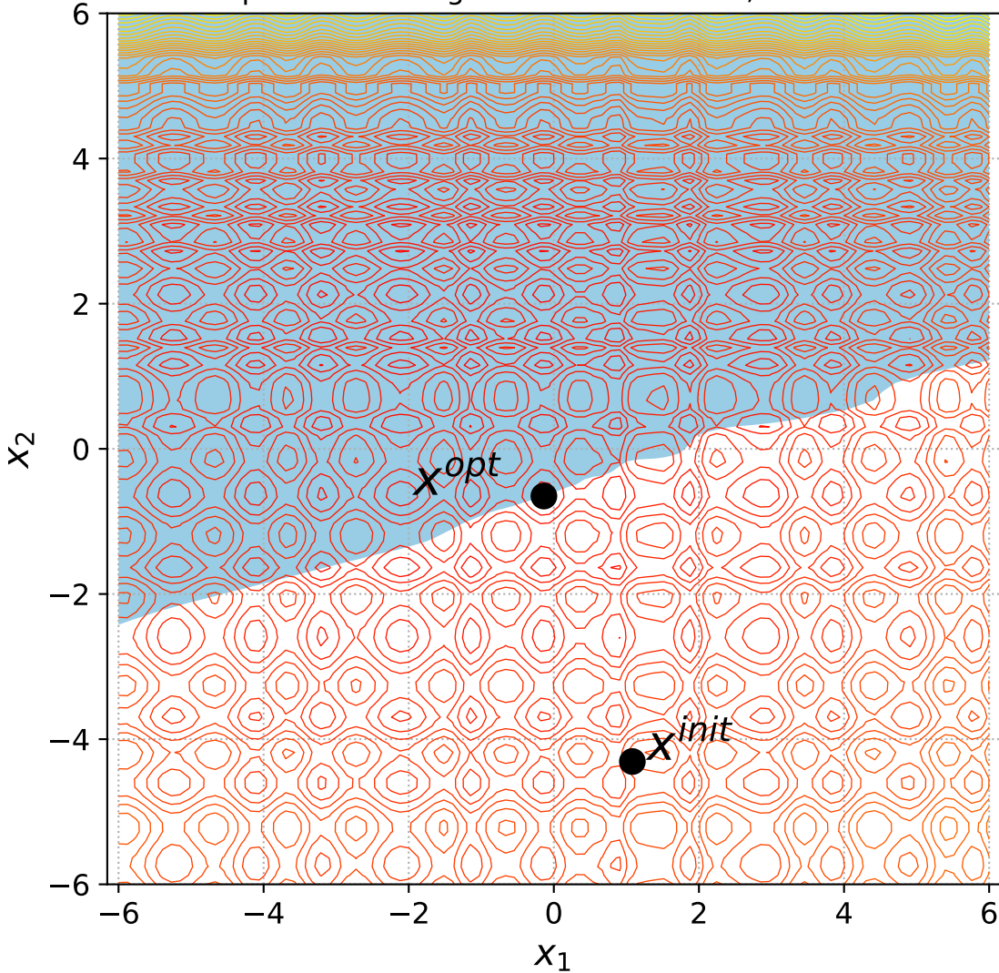
43 Separable Rastrigin with 1 constraint, instance=15
