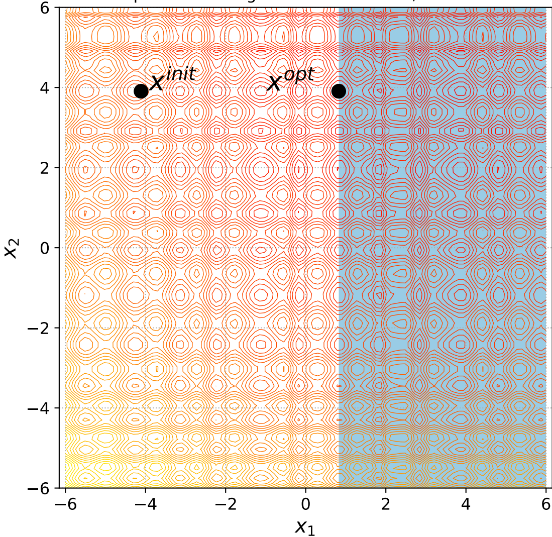
43 Separable Rastrigin with 1 constraint, instance=14
