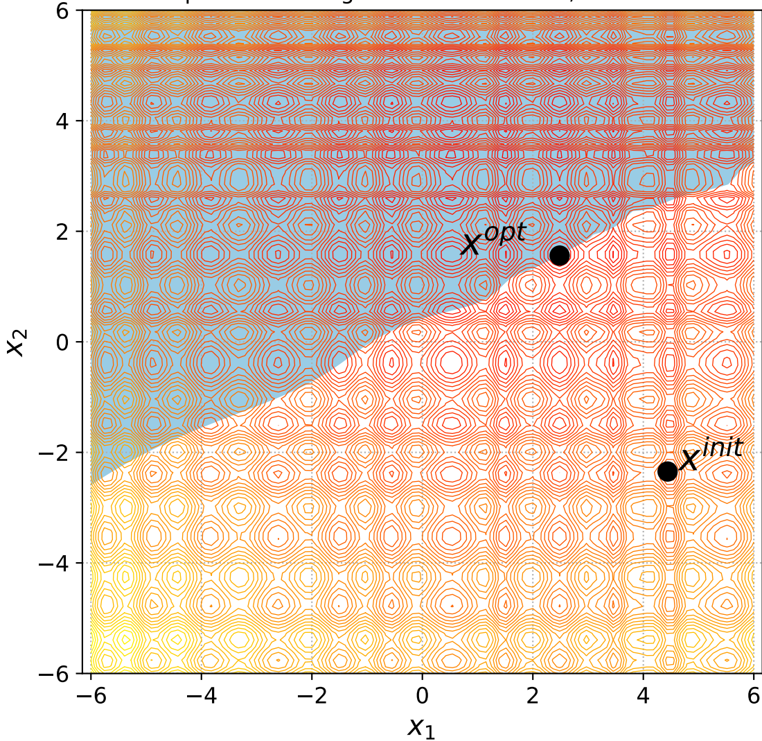
43 Separable Rastrigin with 1 constraint, instance=12
