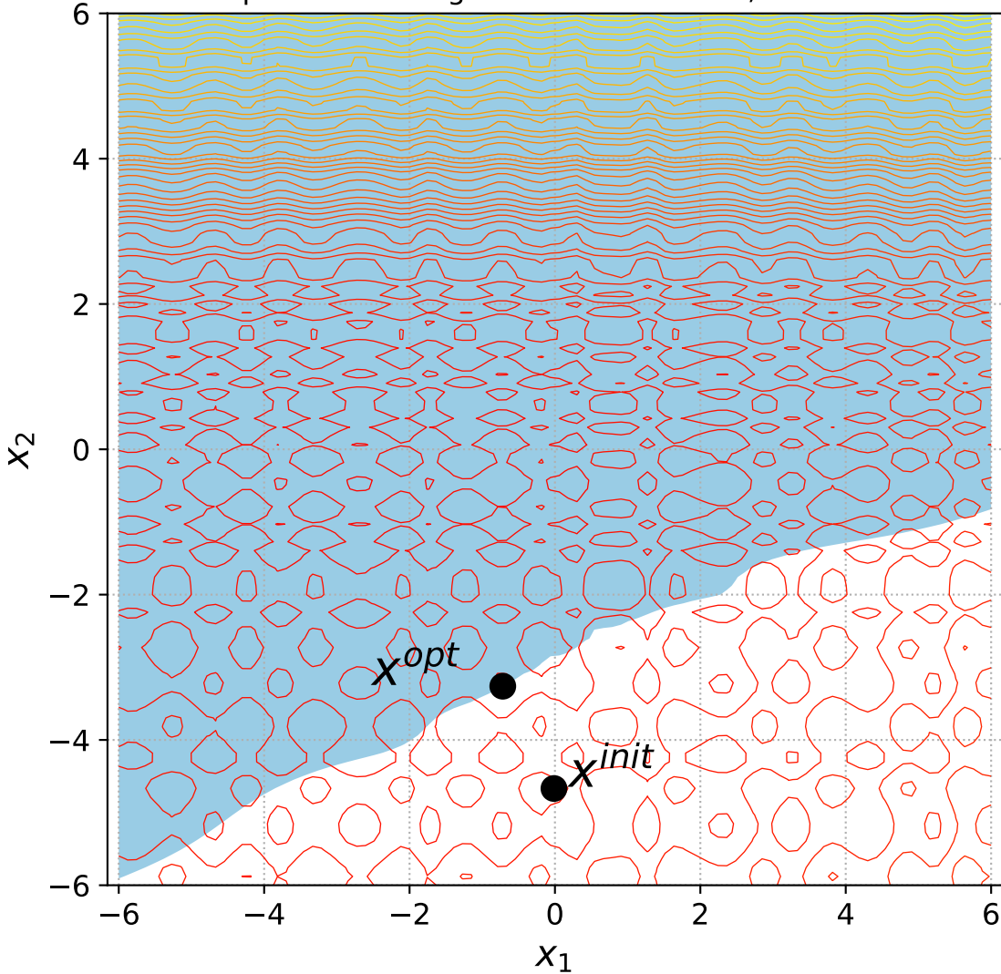
43 Separable Rastrigin with 1 constraint, instance=11
