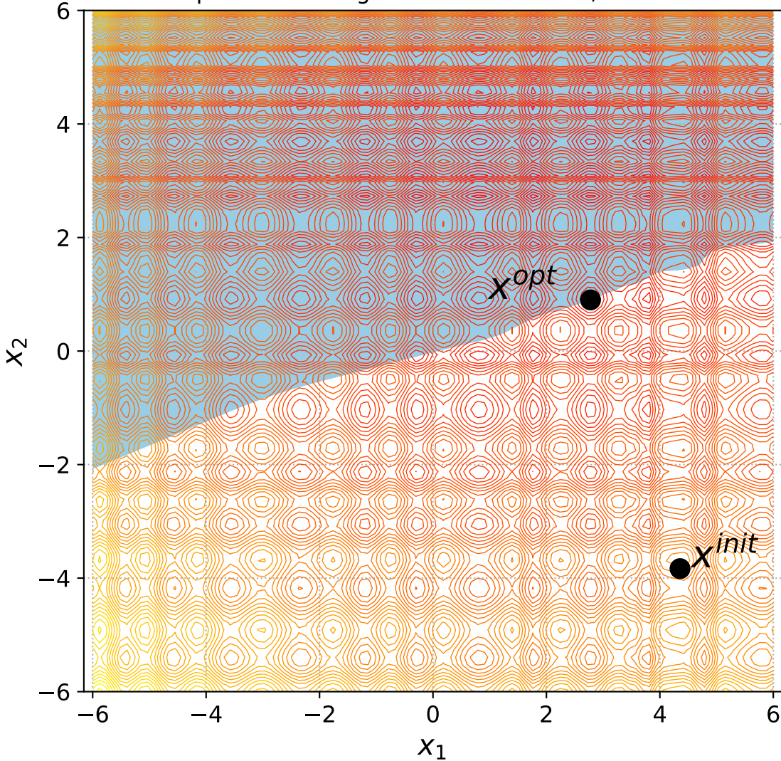
43 Separable Rastrigin with 1 constraint, instance=9
