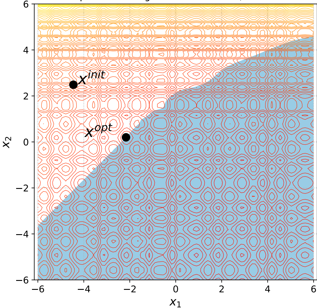
43 Separable Rastrigin with 1 constraint, instance=8
