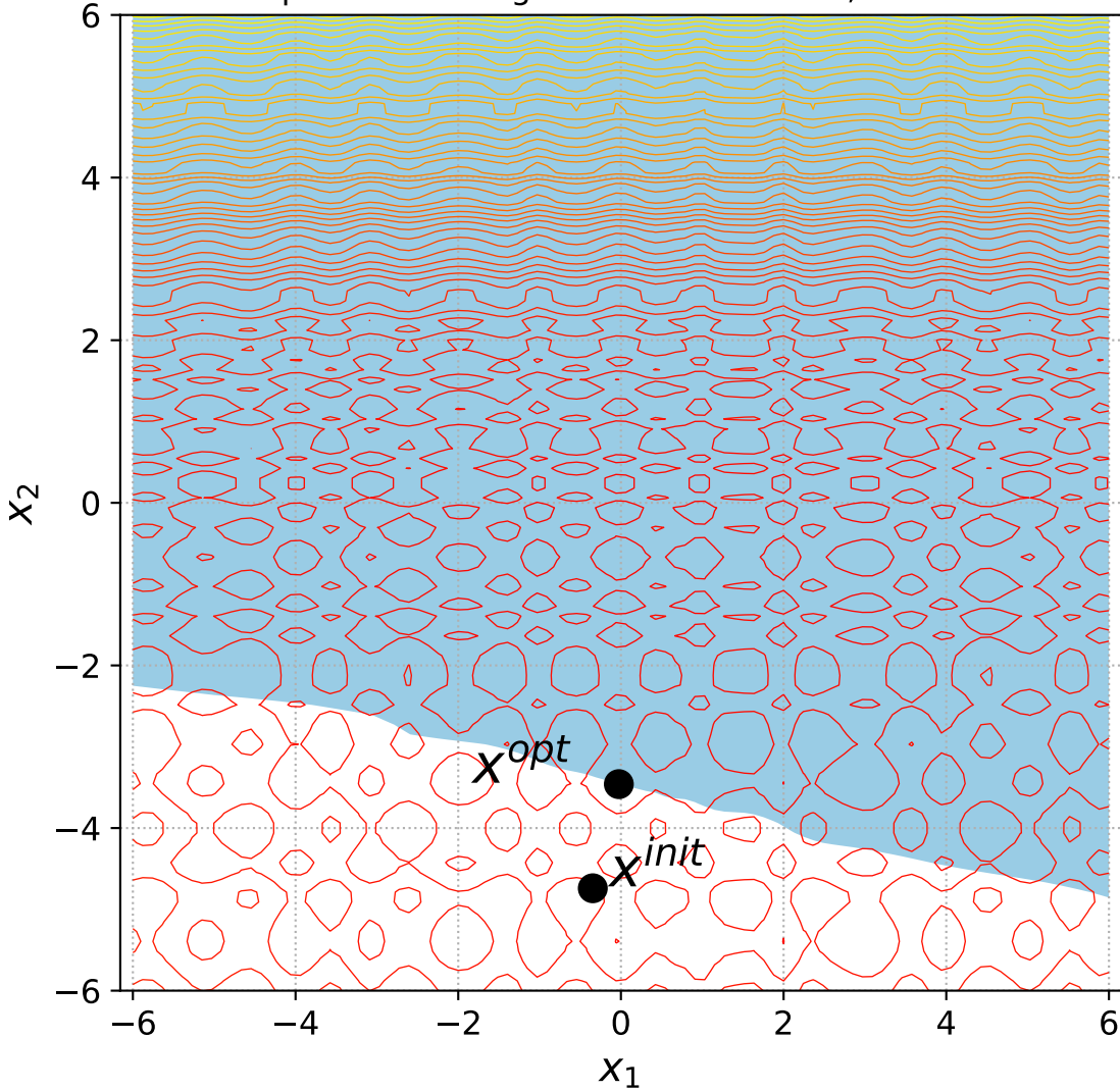
43 Separable Rastrigin with 1 constraint, instance=7
