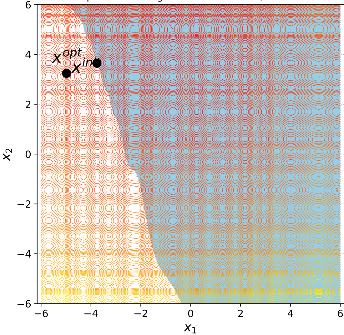
43 Separable Rastrigin with 1 constraint, instance=6
