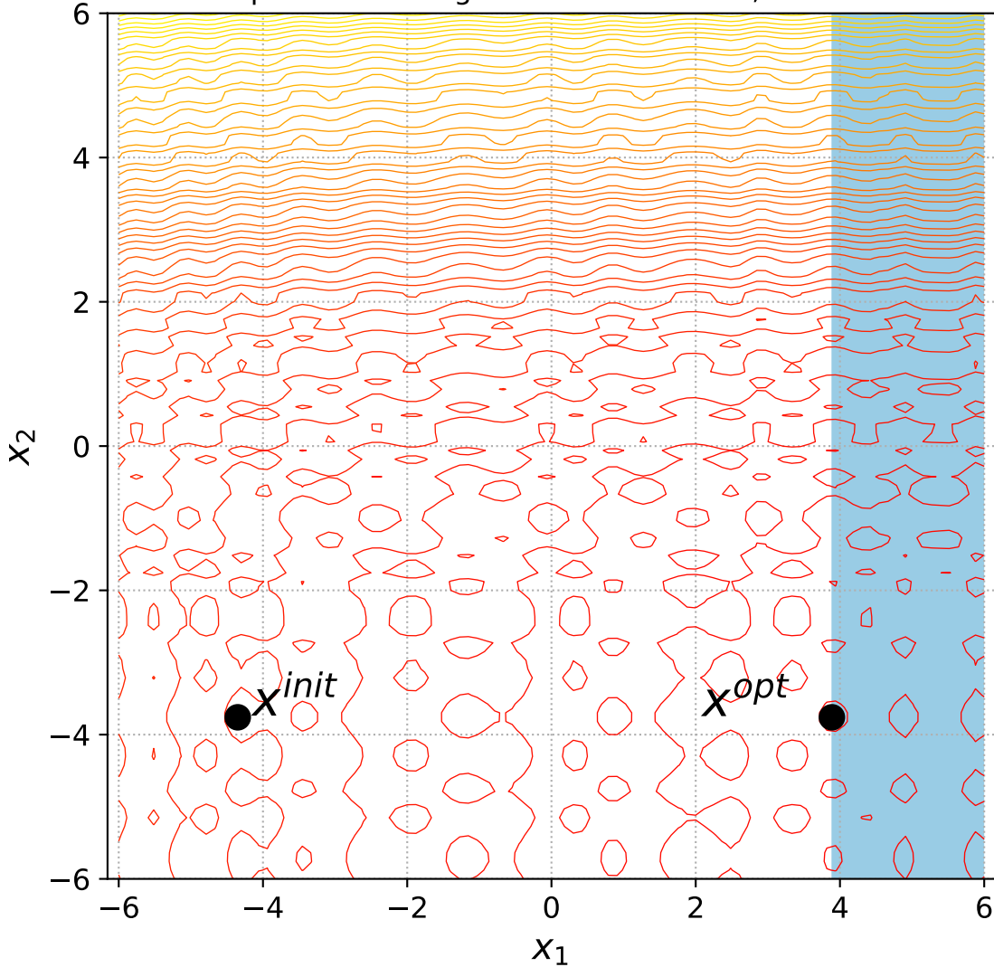
43 Separable Rastrigin with 1 constraint, instance=5
