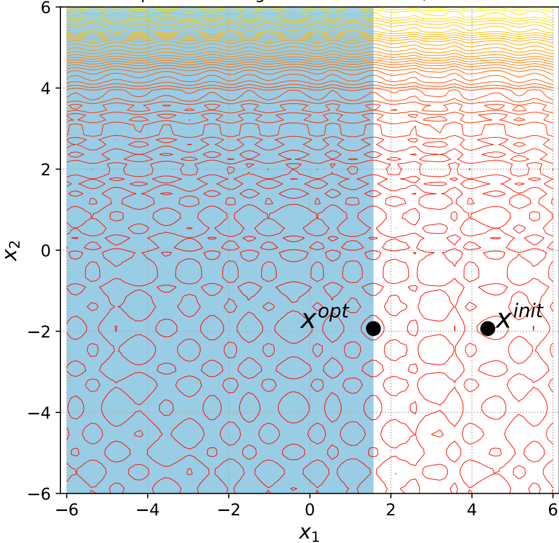
43 Separable Rastrigin with 1 constraint, instance=4
