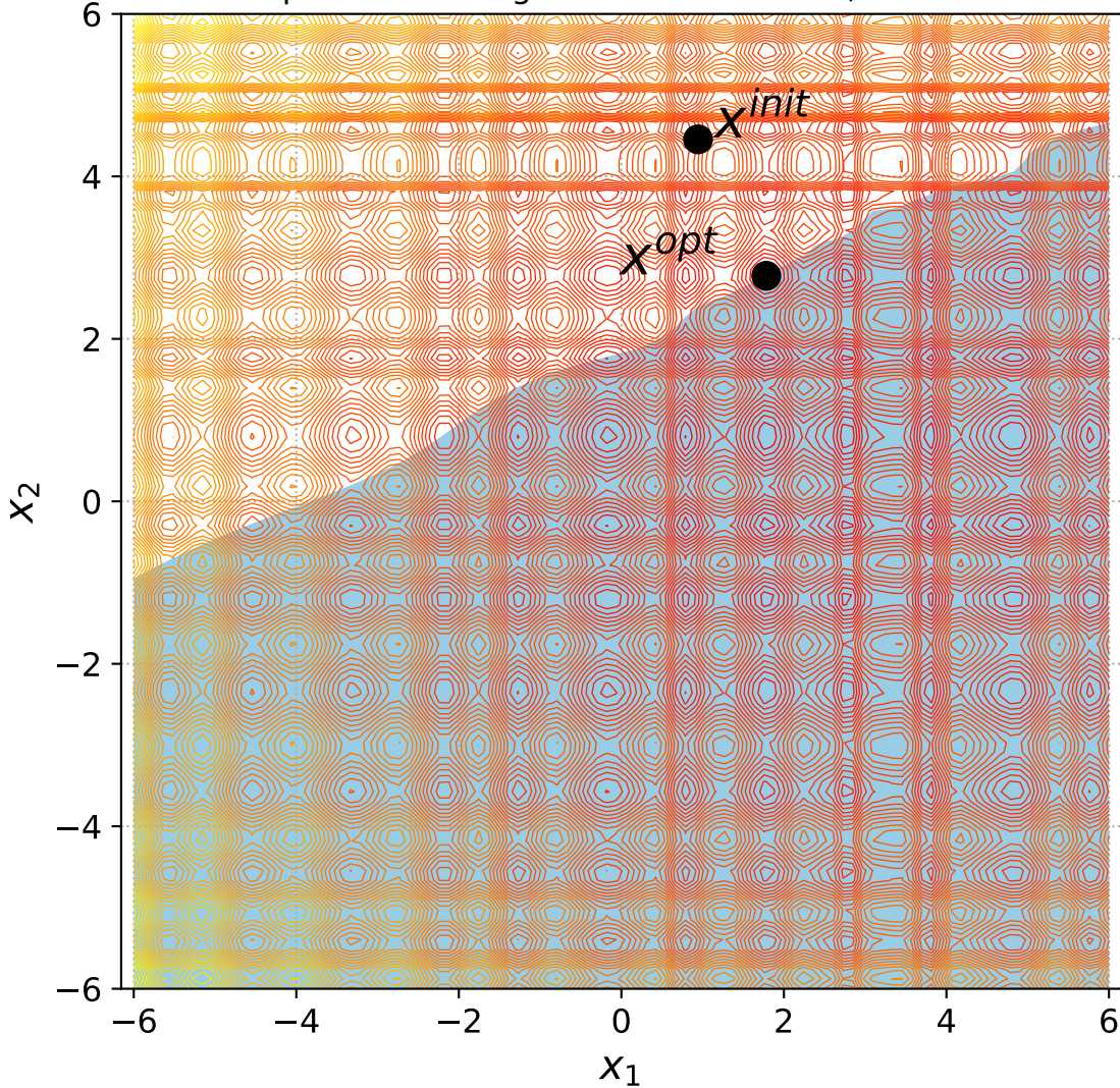
43 Separable Rastrigin with 1 constraint, instance=2
