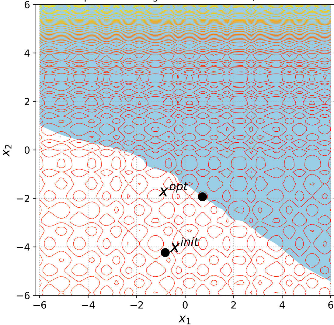
43 Separable Rastrigin with 1 constraint, instance=1
