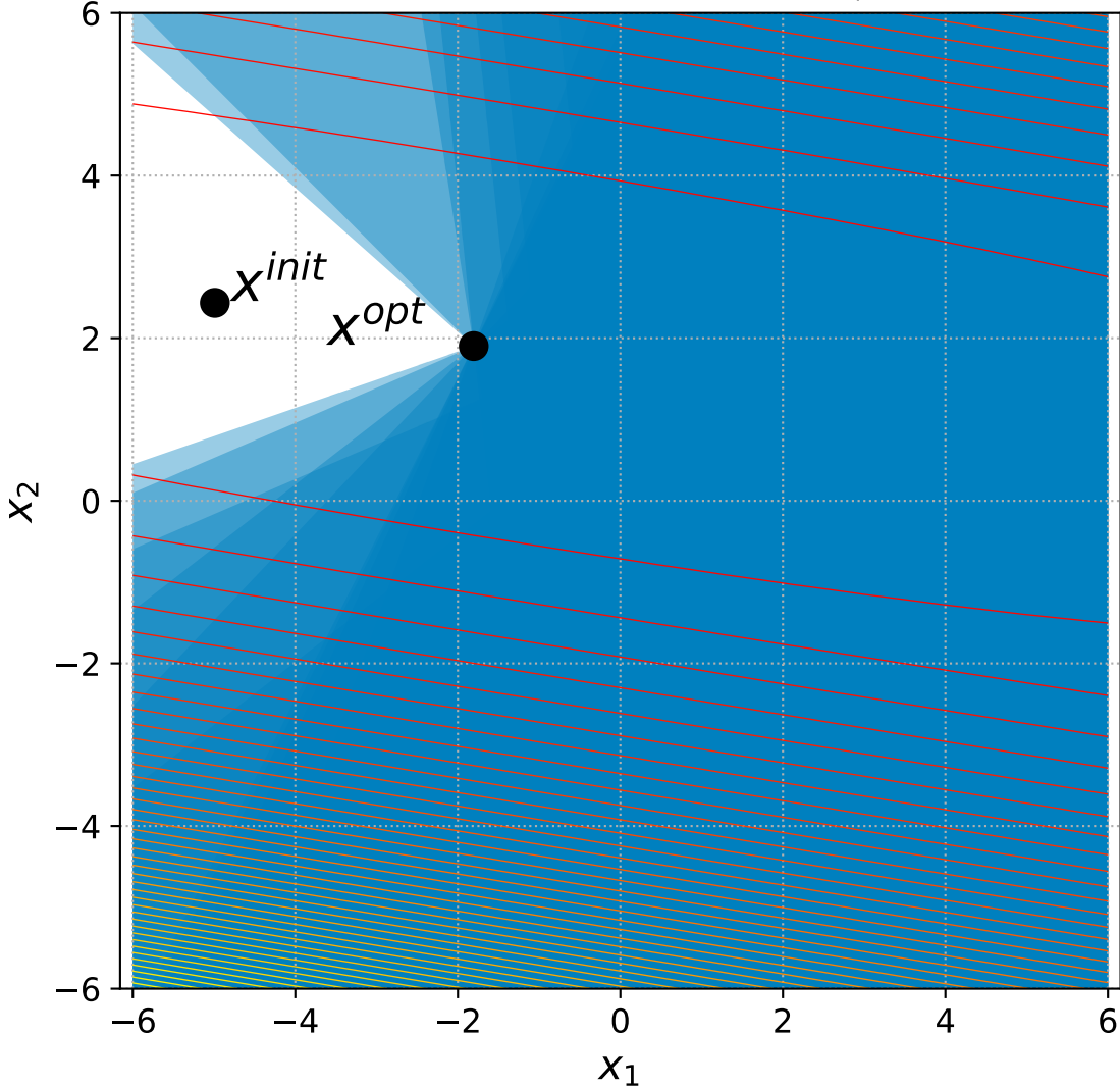
42 Different Powers with 6+3n constraints, instance=14
