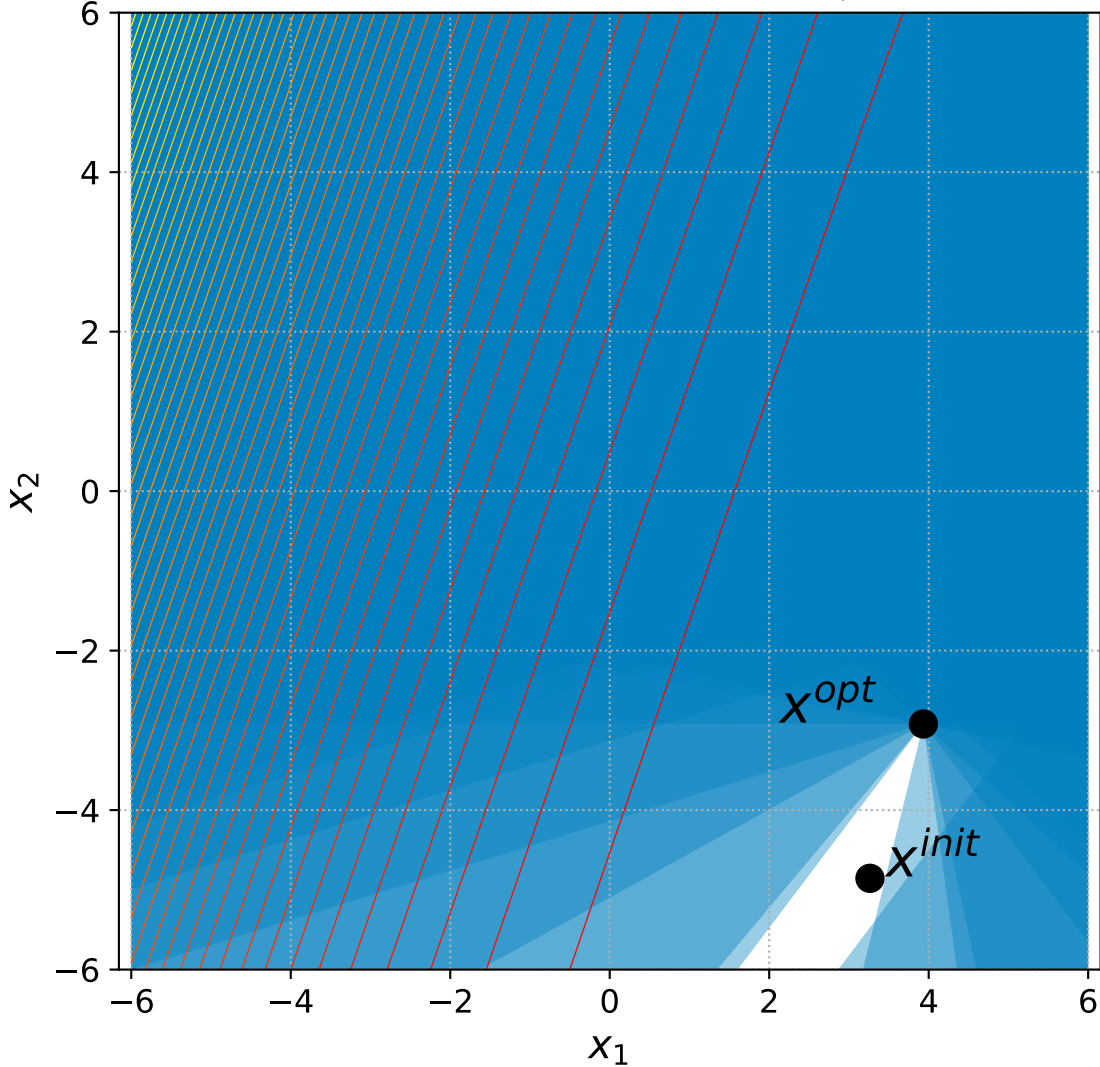
42 Different Powers with 6+3n constraints, instance=11
