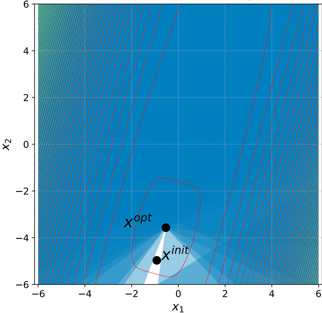
42 Different Powers with 6+3n constraints, instance=8
