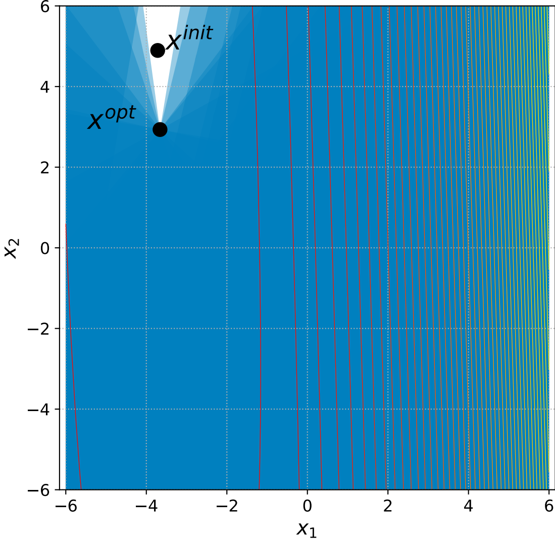
42 Different Powers with 6+3n constraints, instance=6
