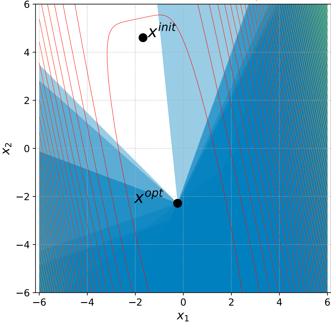
42 Different Powers with 6+3n constraints, instance=4
