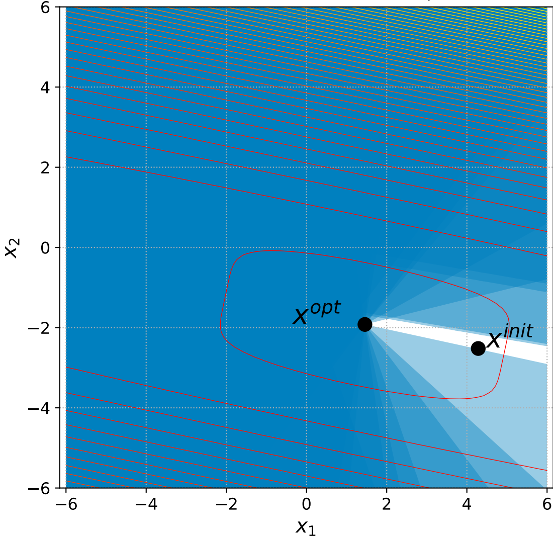
42 Different Powers with 6+3n constraints, instance=1
