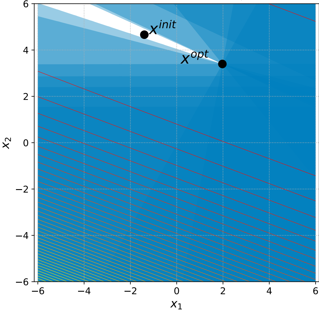
41 Different Powers with 6+n constraints, instance=15
