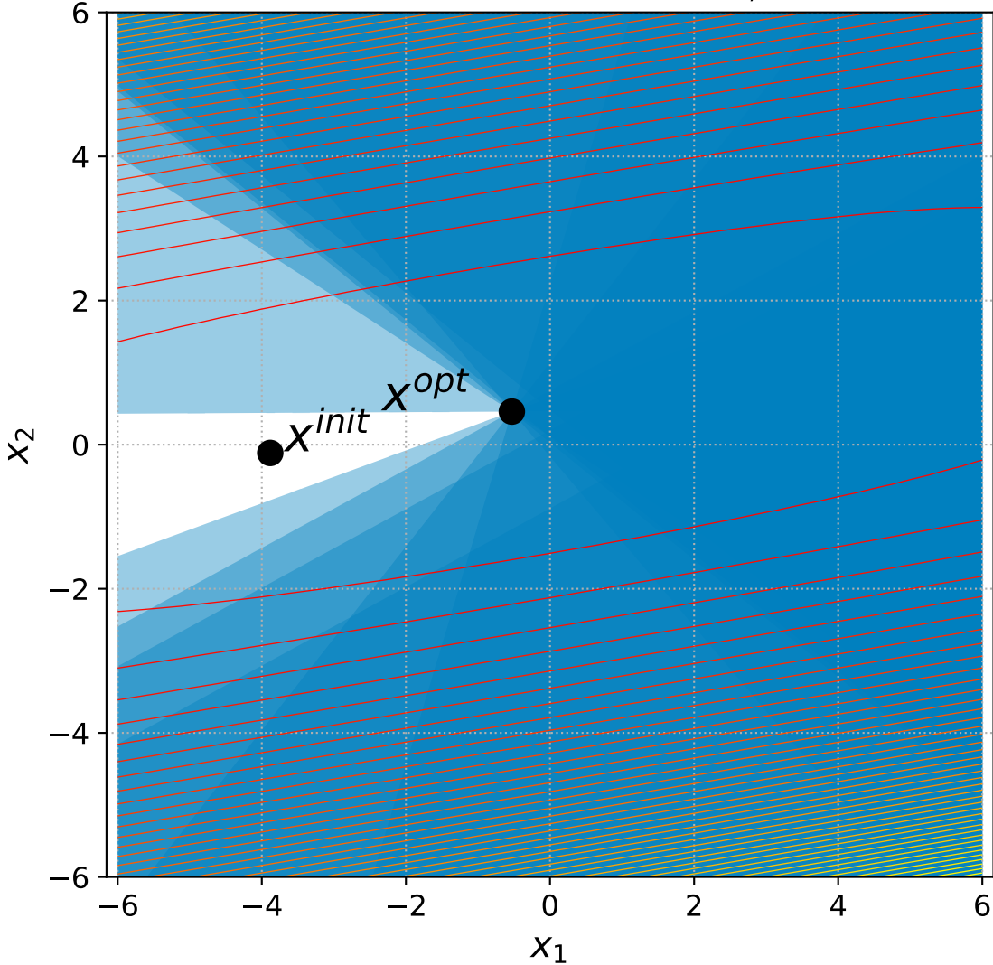
41 Different Powers with 6+n constraints, instance=12
