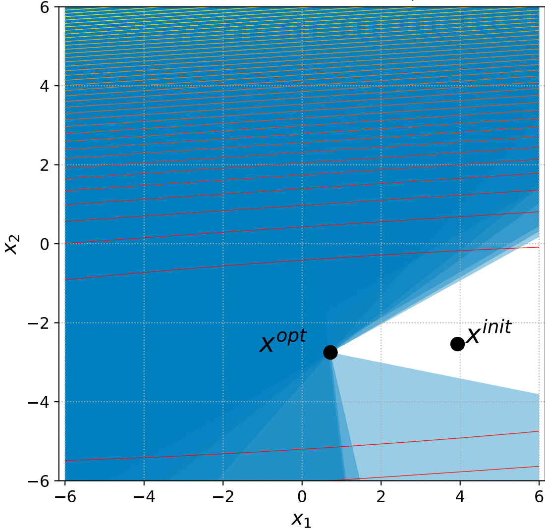
41 Different Powers with 6+n constraints, instance=11
