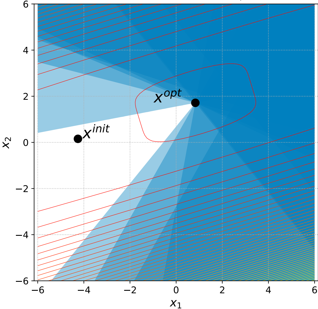
41 Different Powers with 6+n constraints, instance=10
