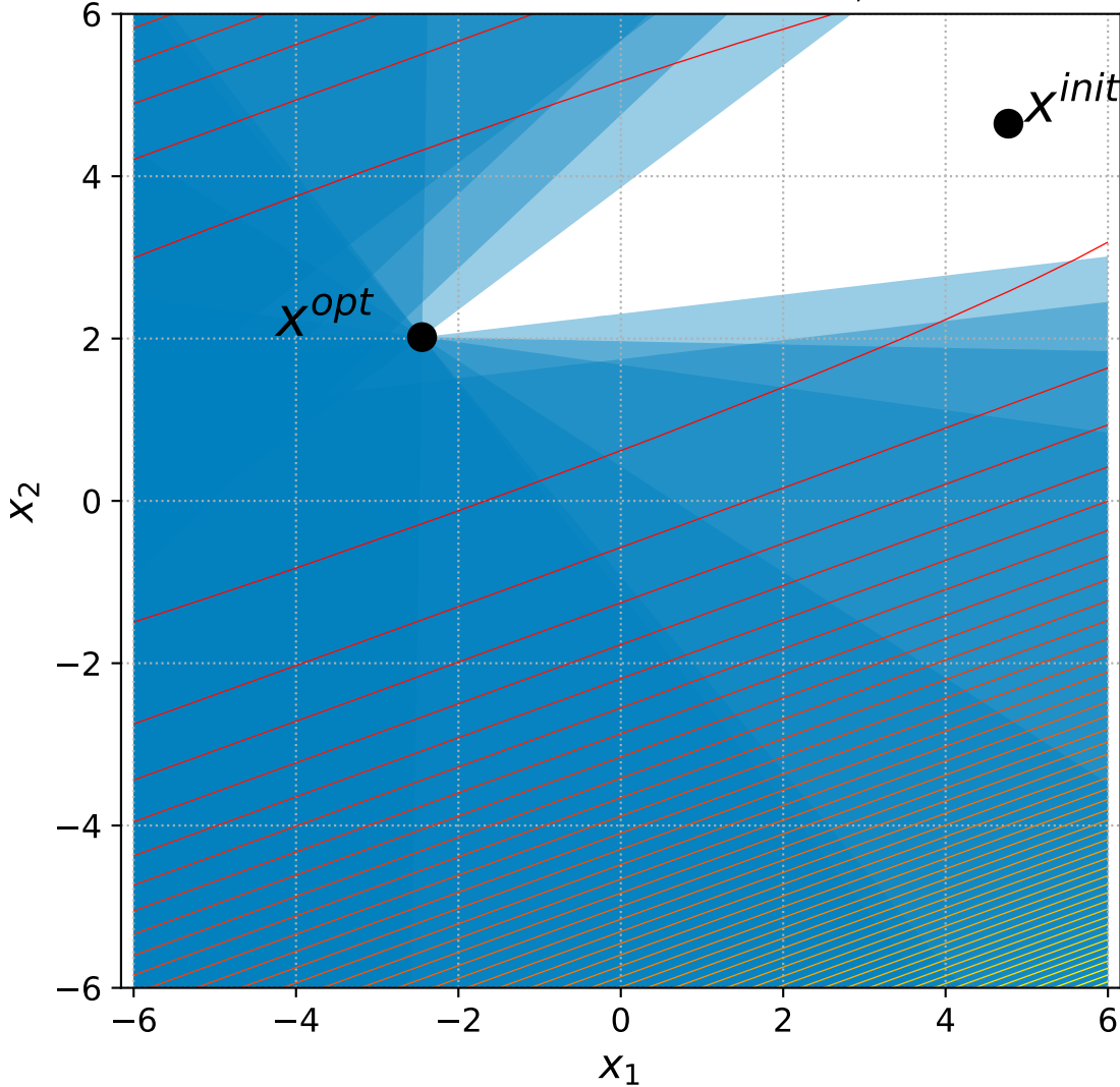
41 Different Powers with 6+n constraints, instance=9
