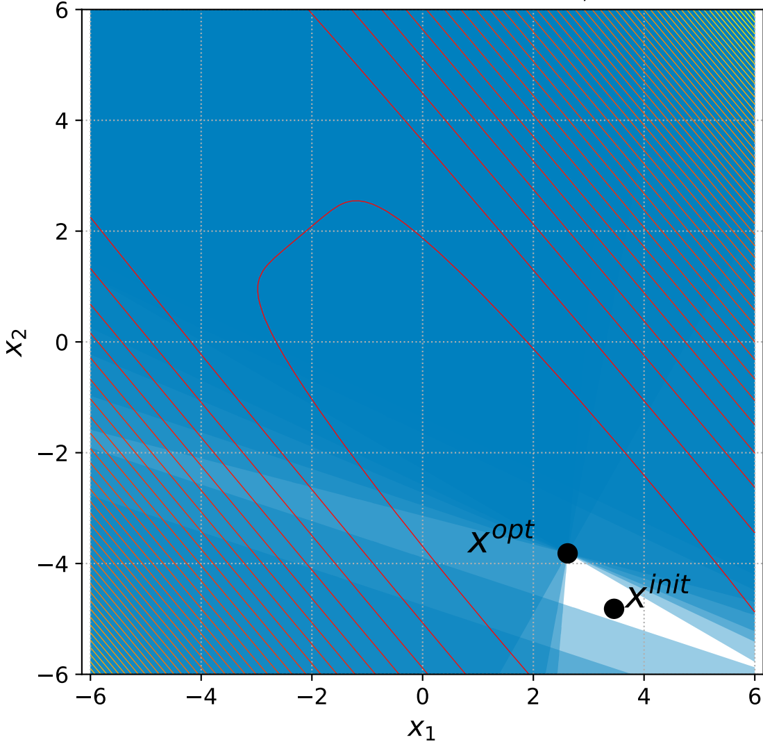
41 Different Powers with 6+n constraints, instance=5
