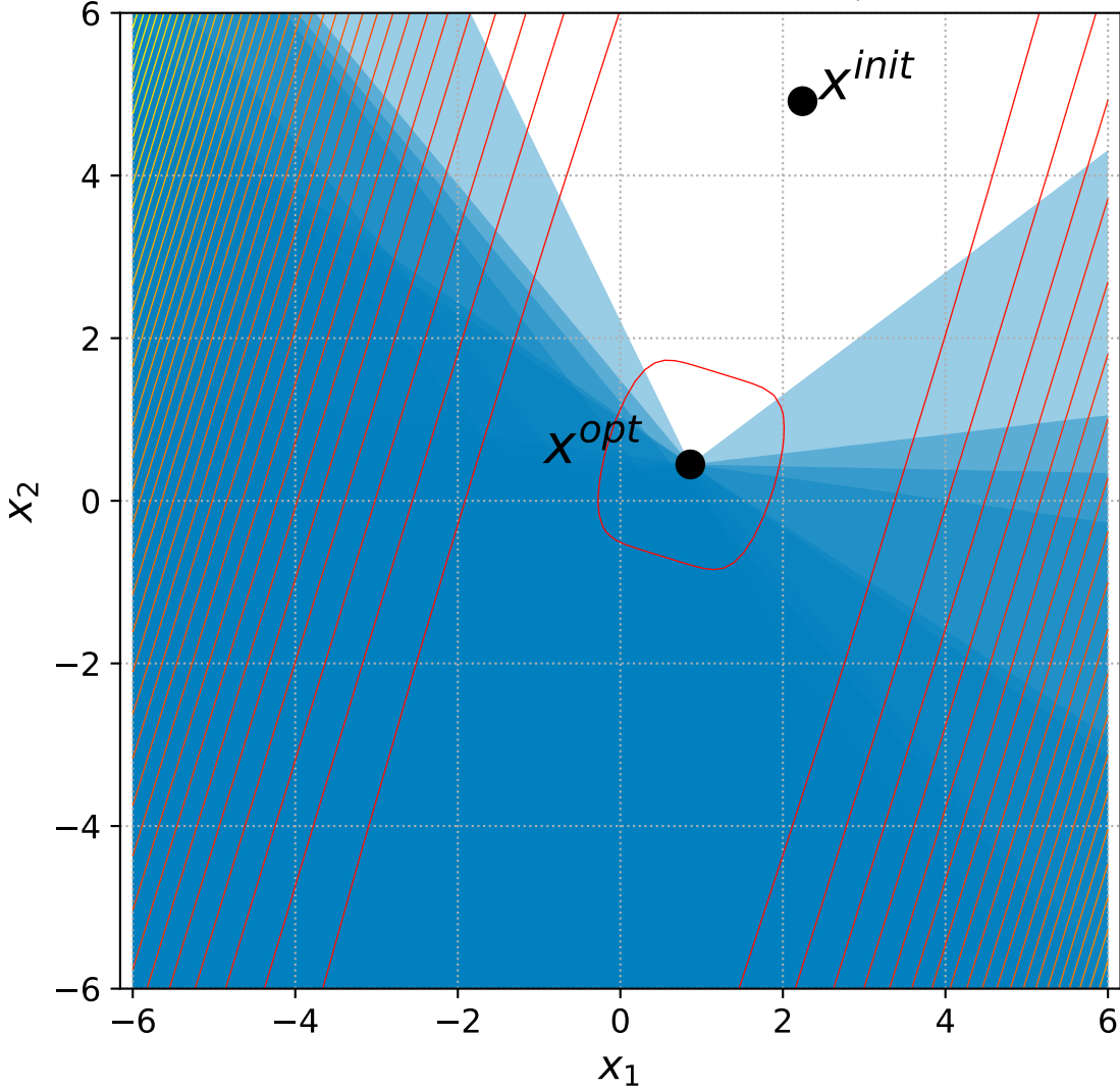
41 Different Powers with 6+n constraints, instance=4
