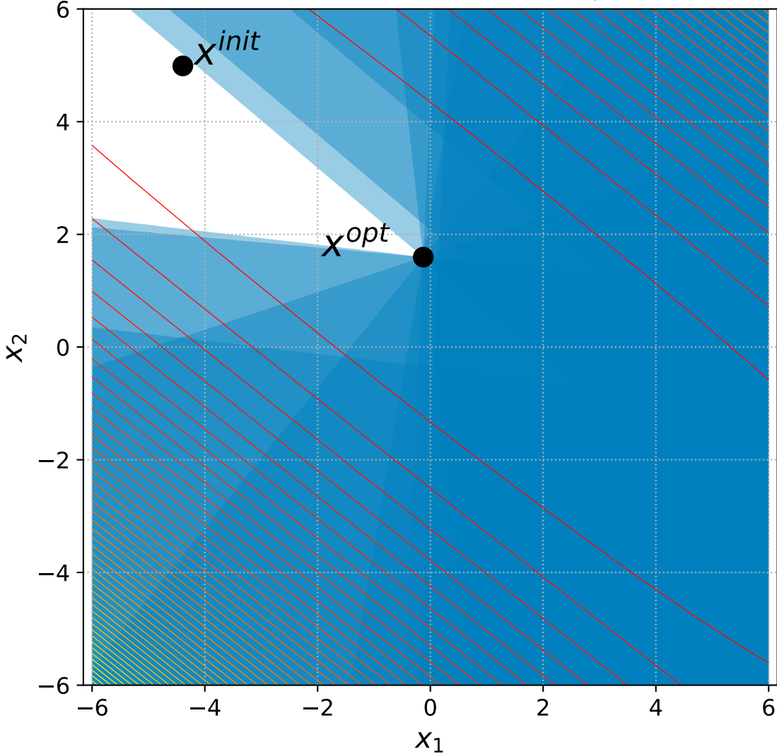
41 Different Powers with 6+n constraints, instance=3
