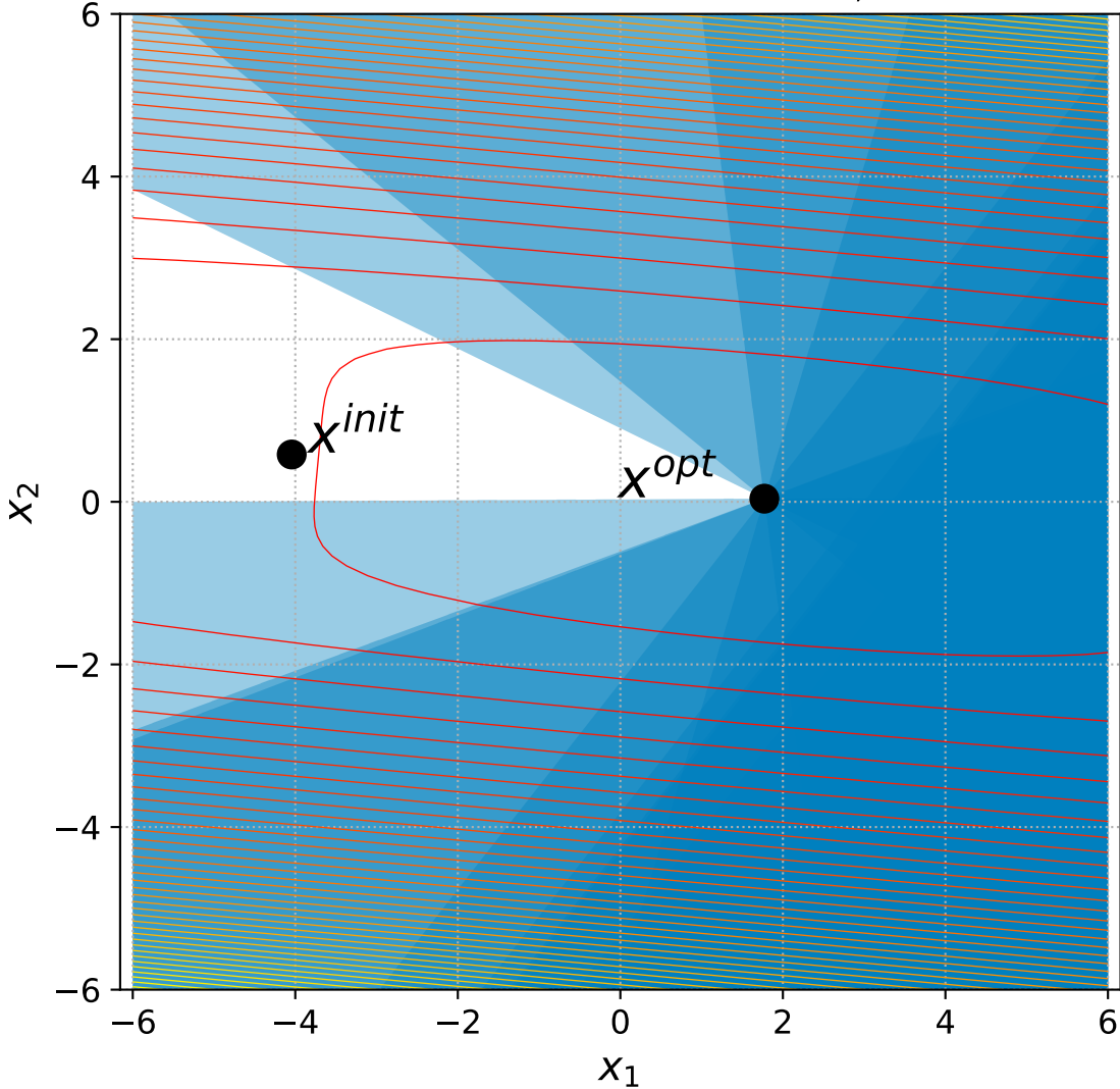
41 Different Powers with 6+n constraints, instance=2
