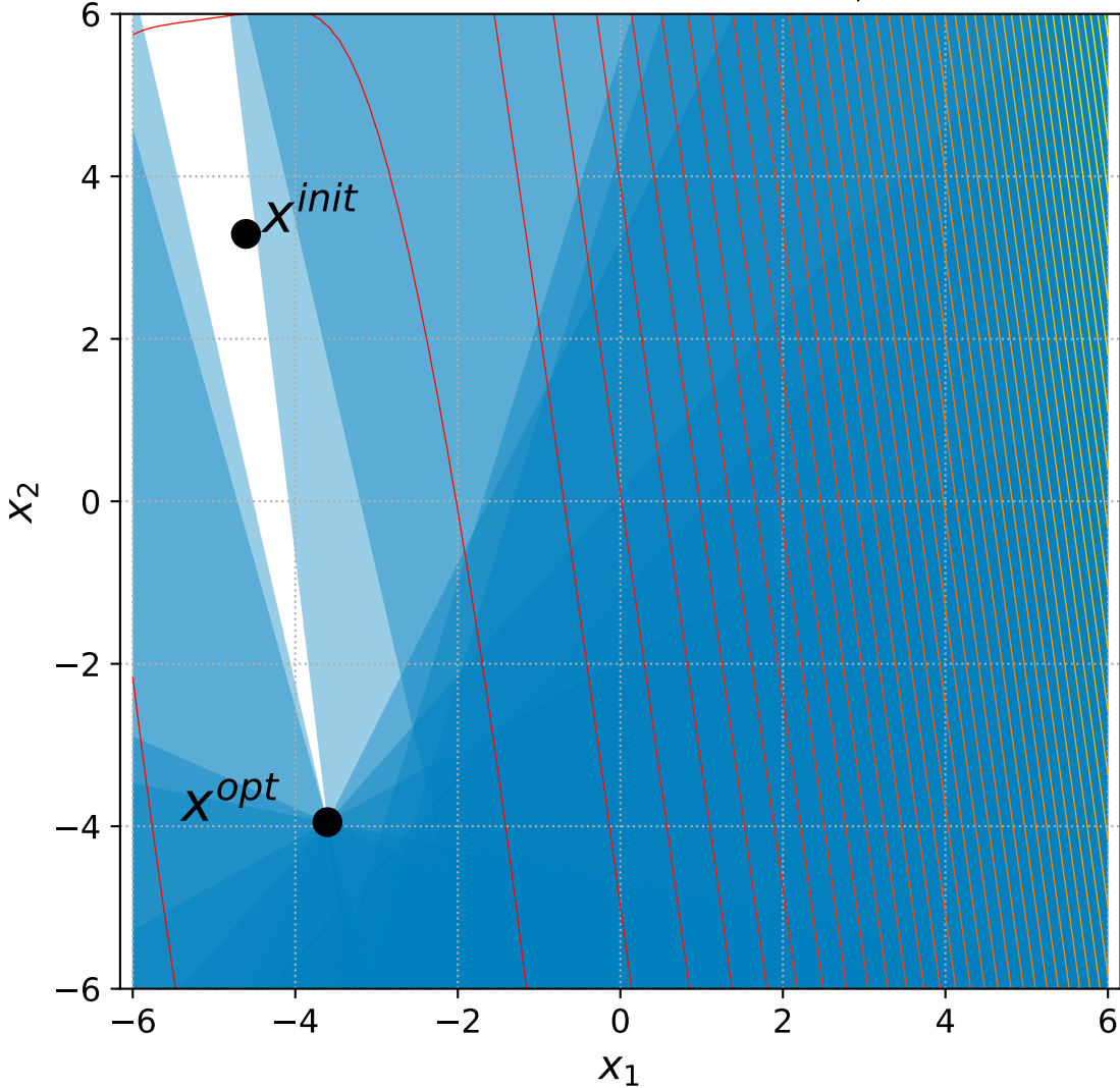
41 Different Powers with 6+n constraints, instance=1
