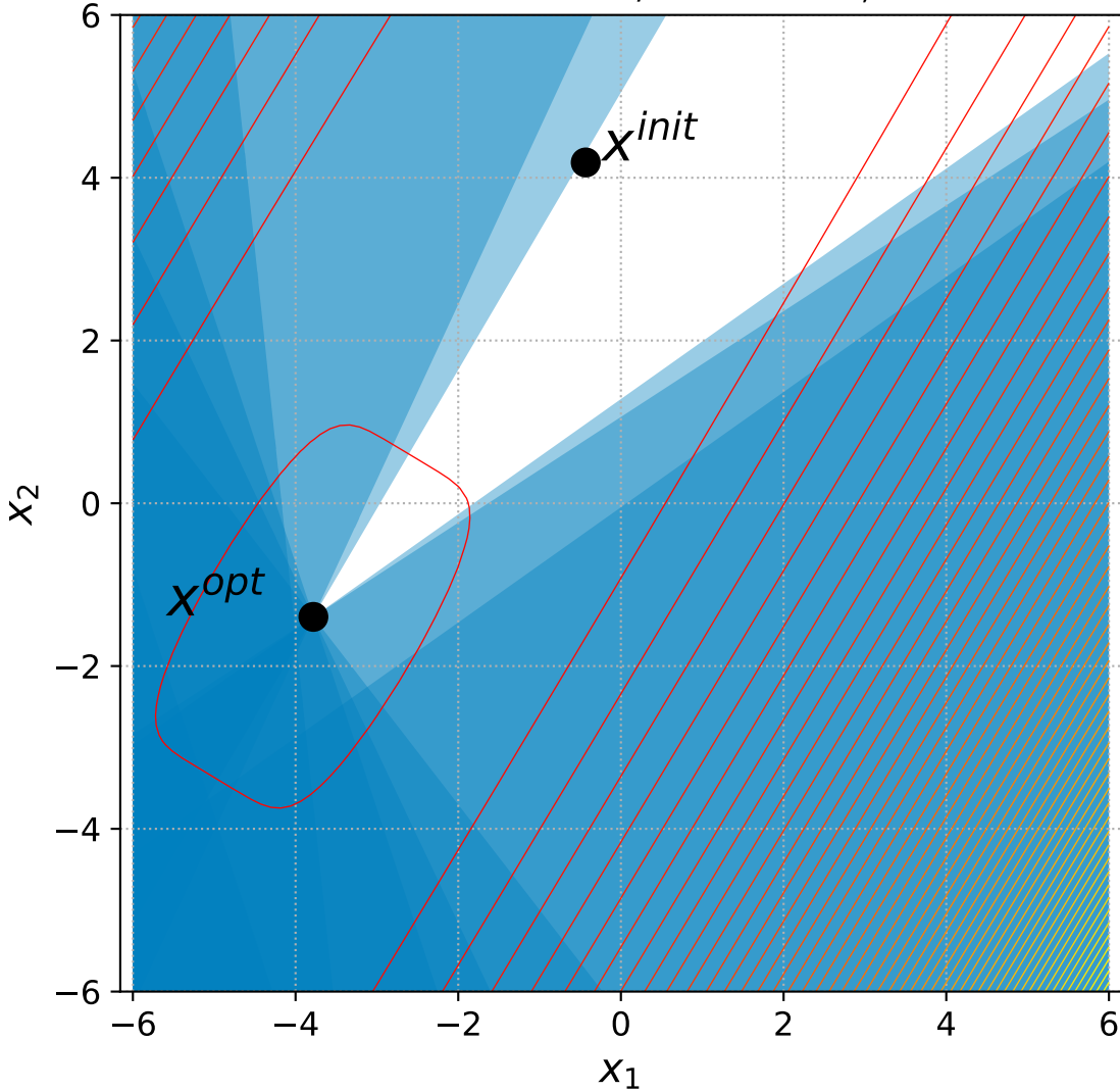
40 Different Powers with 6+n/2 constraints, instance=14
