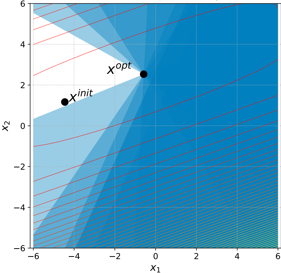
40 Different Powers with 6+n/2 constraints, instance=11
