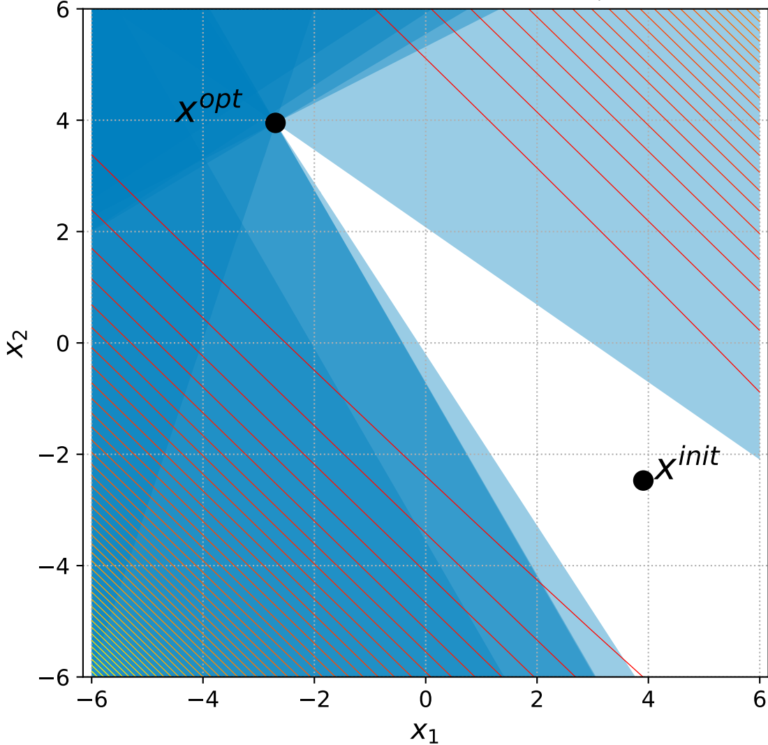
40 Different Powers with 6+n/2 constraints, instance=8
