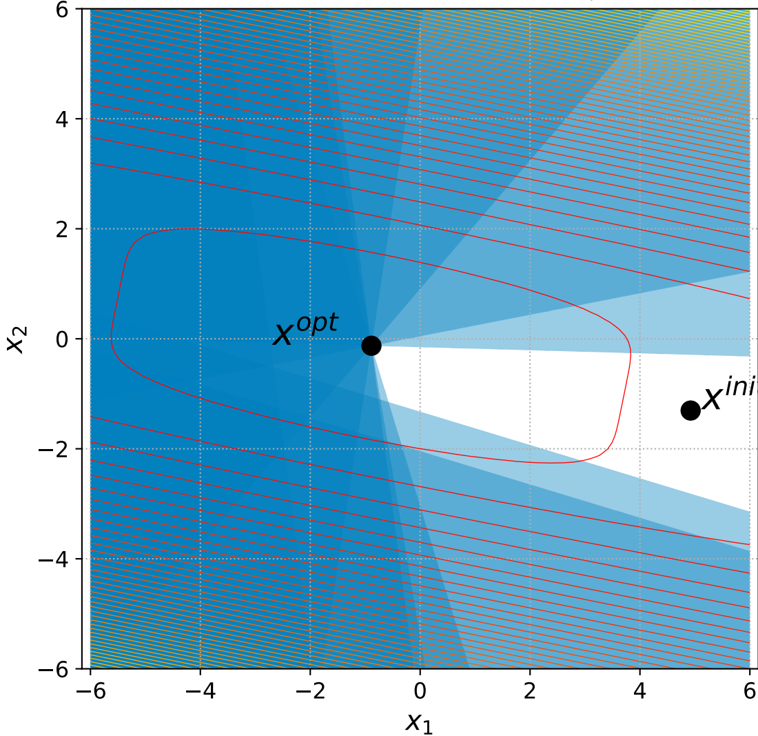
40 Different Powers with 6+n/2 constraints, instance=7
