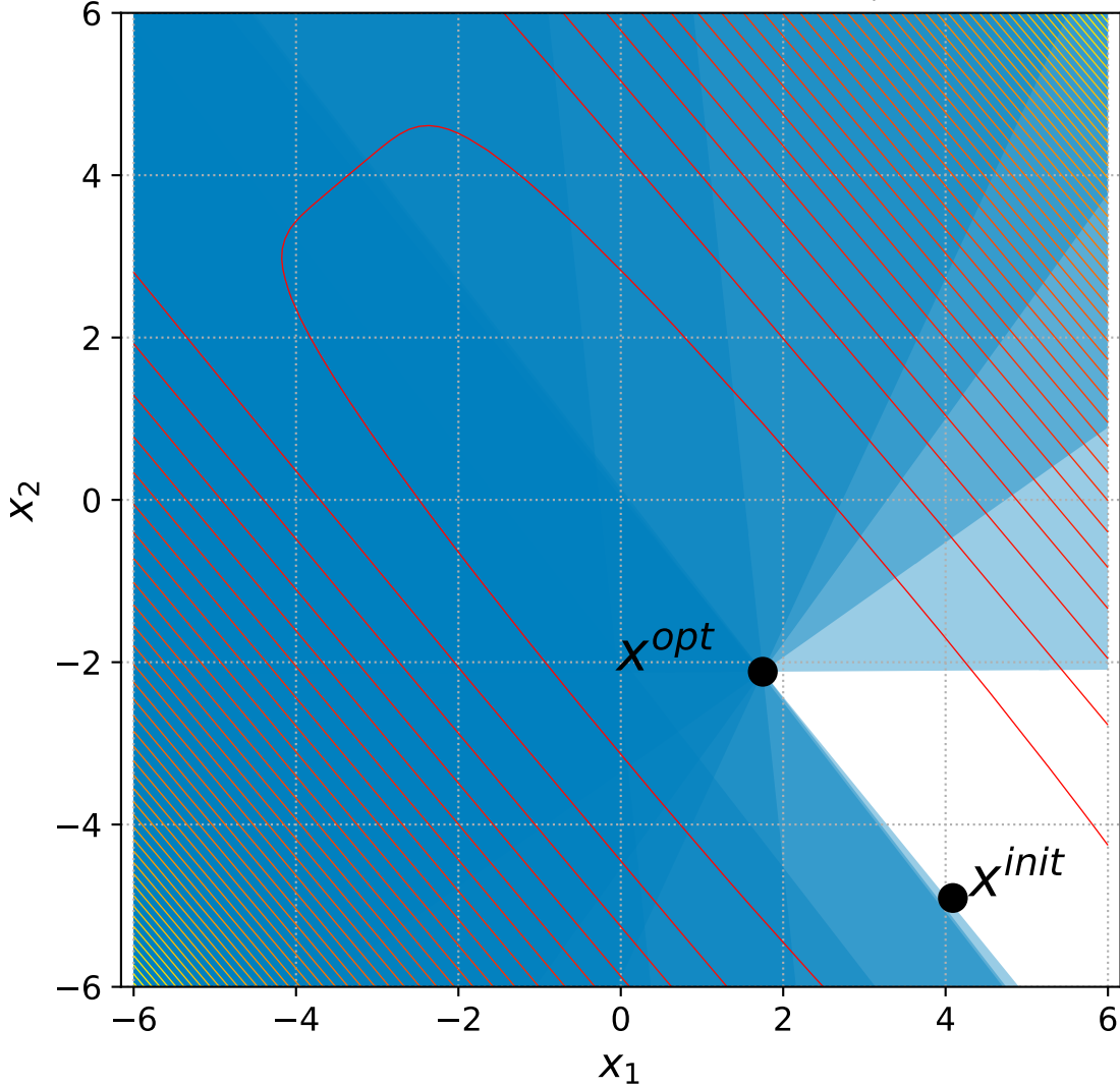
40 Different Powers with 6+n/2 constraints, instance=4
