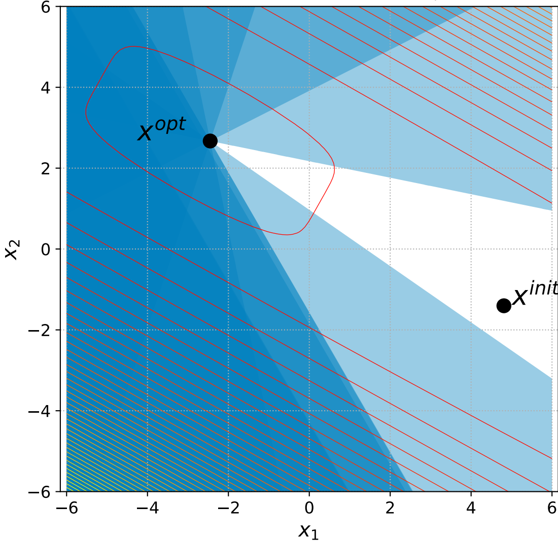
40 Different Powers with 6+n/2 constraints, instance=3
