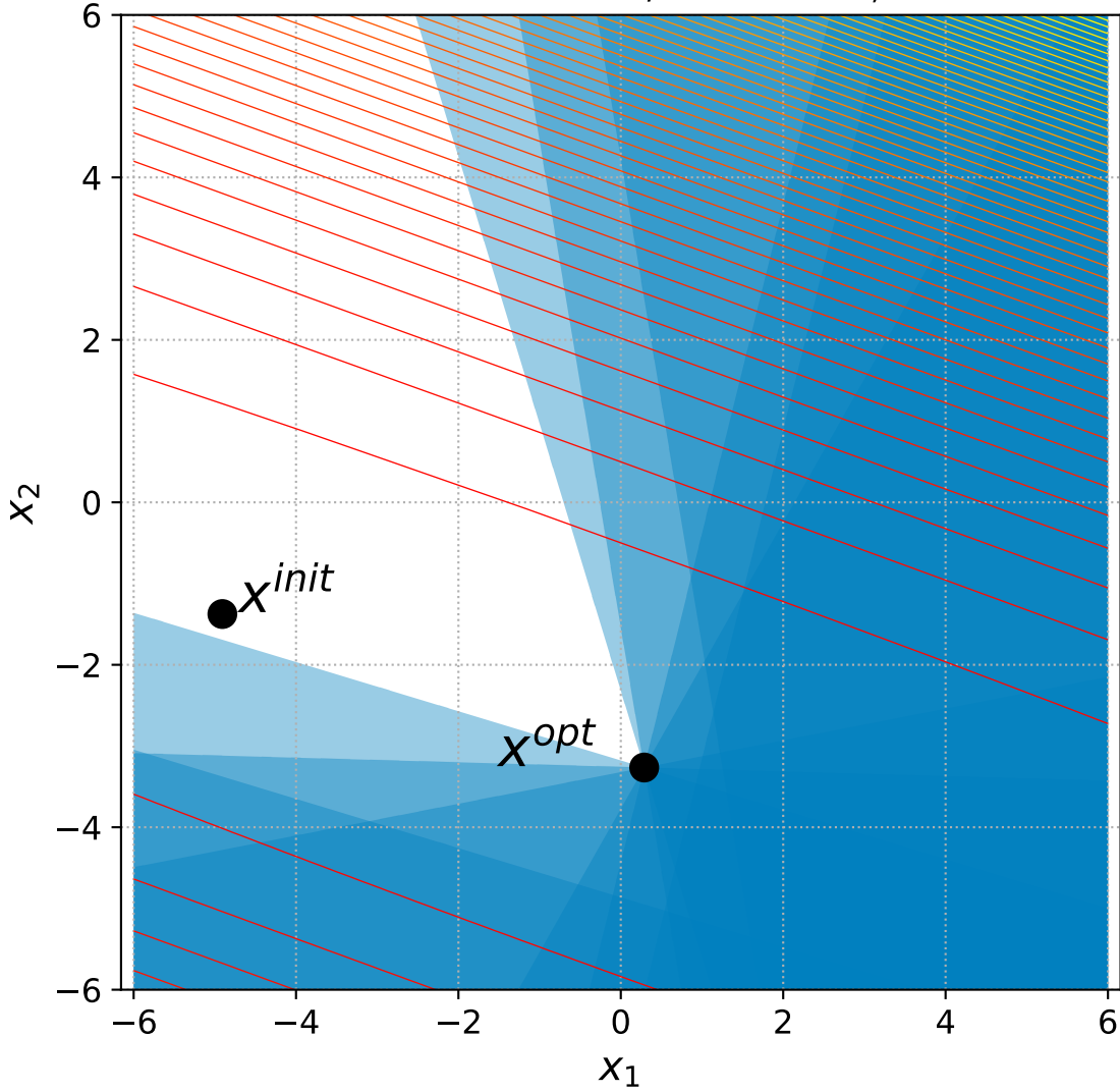
40 Different Powers with 6+n/2 constraints, instance=2
