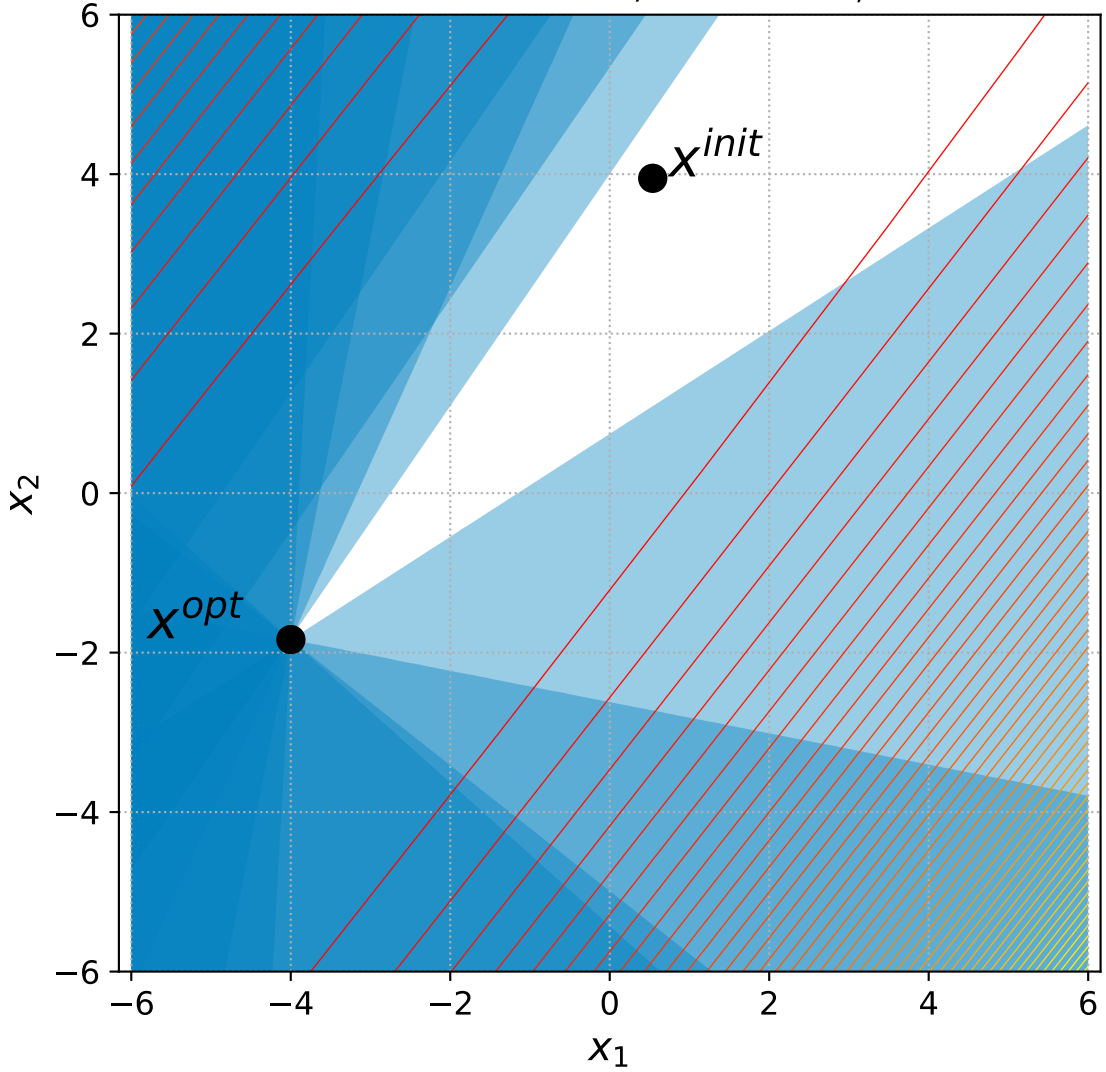
40 Different Powers with 6+n/2 constraints, instance=1
